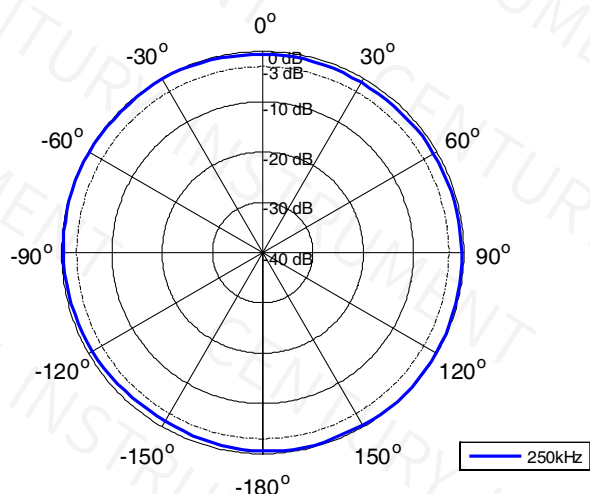
Horizontal directivity pattern
