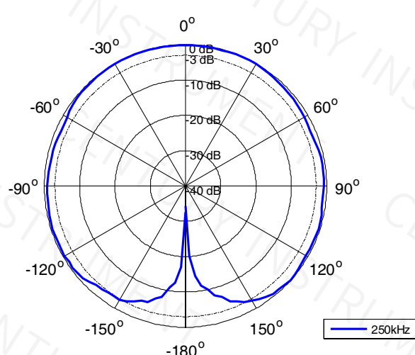
Vertical directivity pattern
